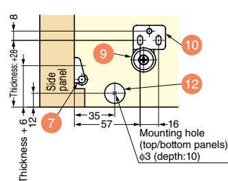
Arrow view b: For roller bracket mounting
