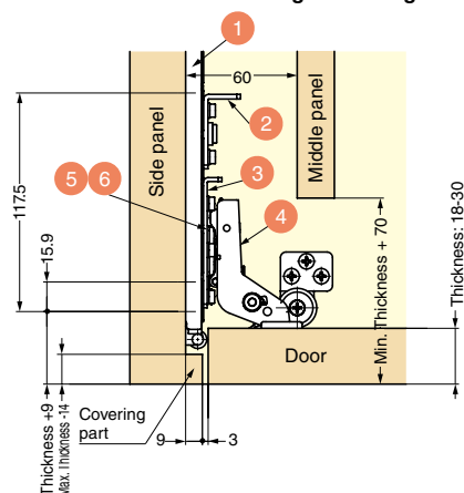
Cross section a: Slide/hinge mounting
