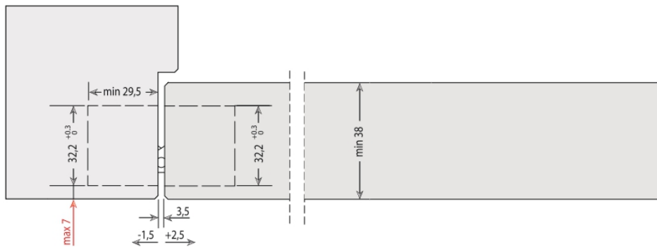
Door cross-section
